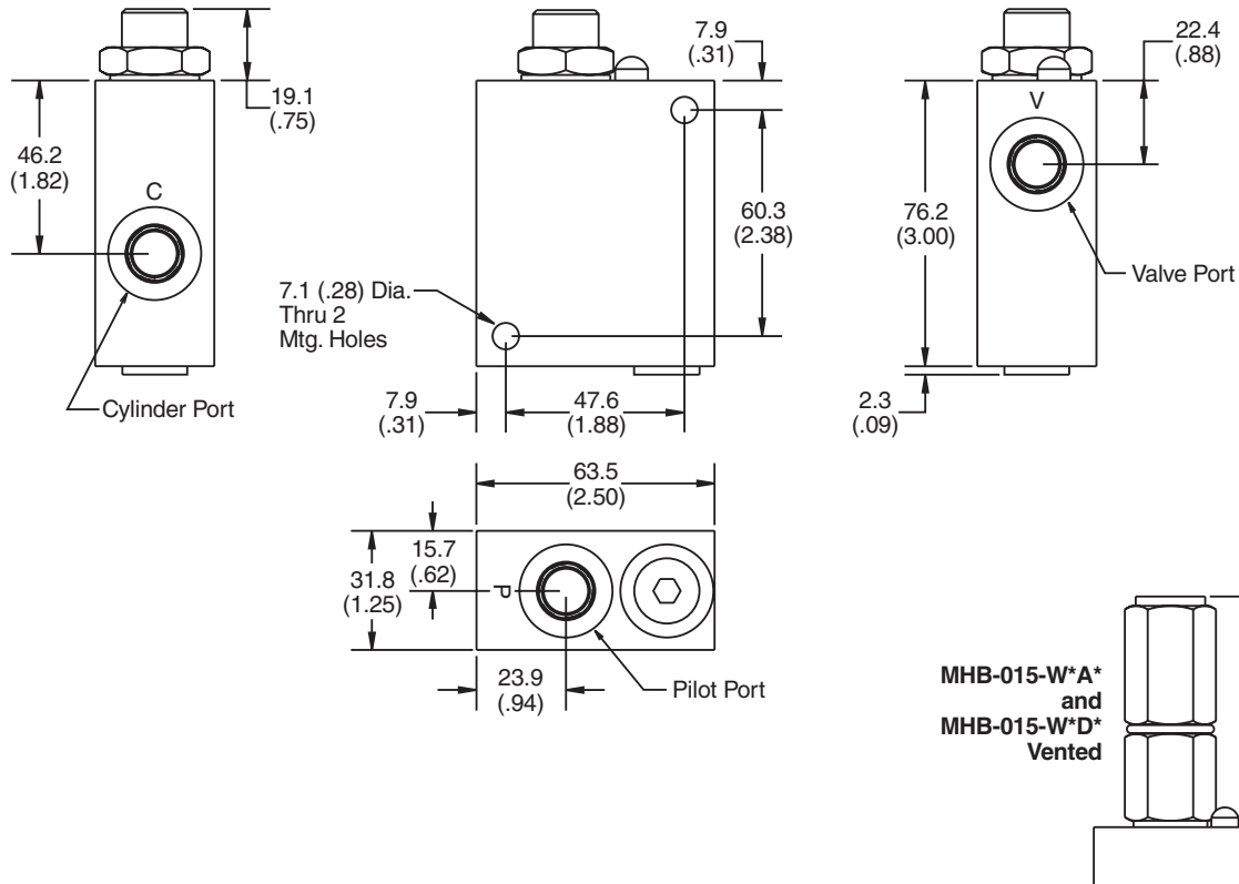
MHB-015-L*A* Non-Vented
