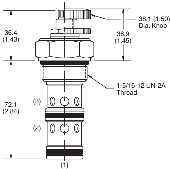
Screw/Knob Version
